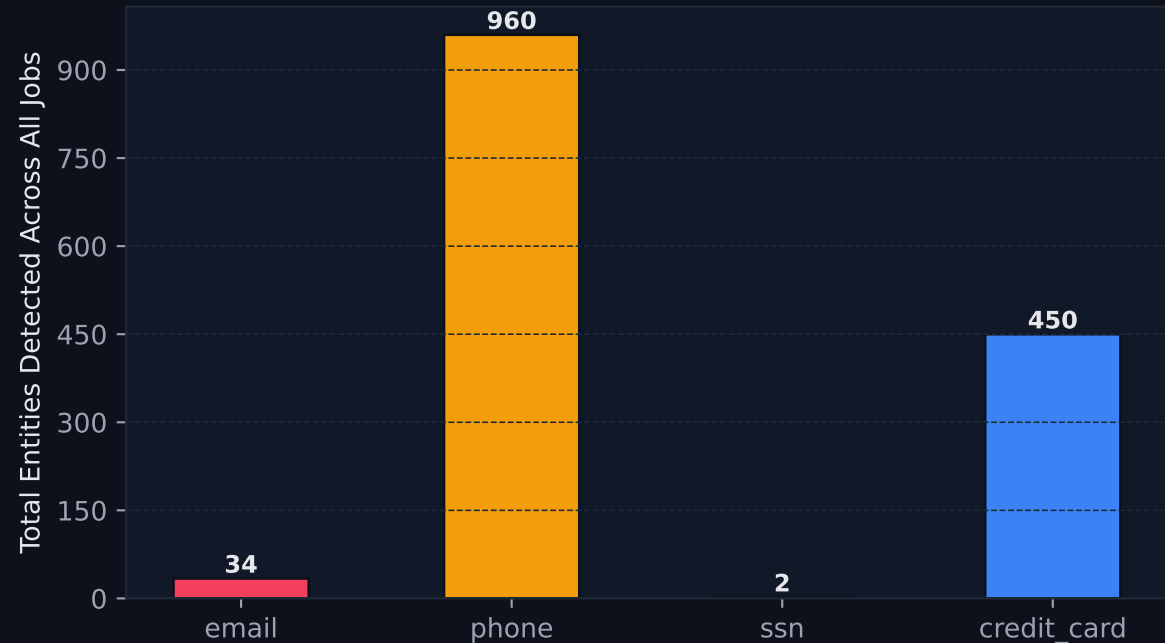
Figure 7 — PII Entity Type Detection Summary
