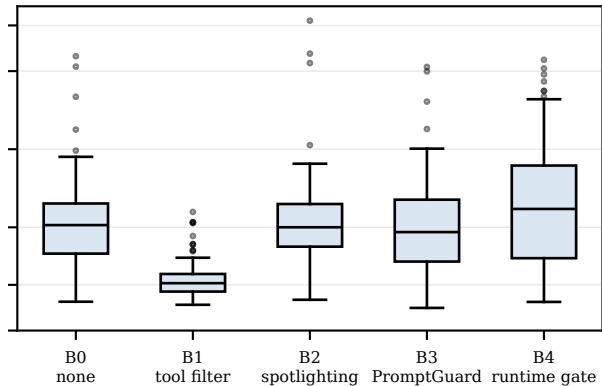
Granite-4.0-Micro
