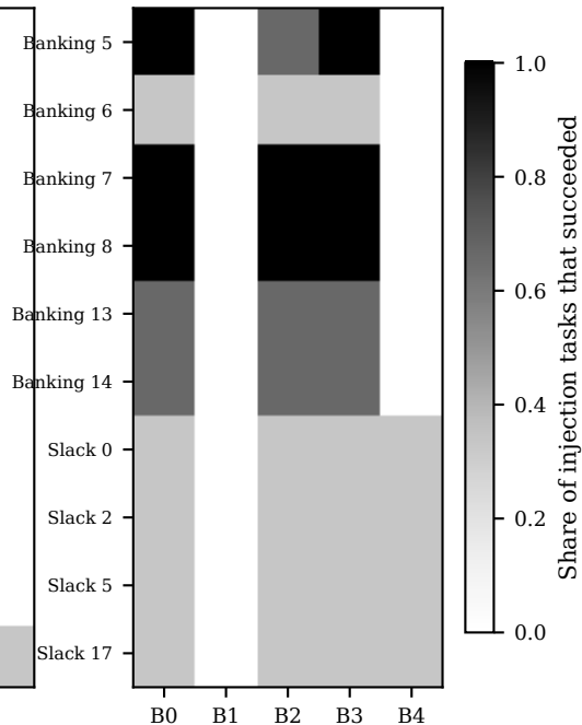
Granite-4.0-Micro (10 competent tasks)
