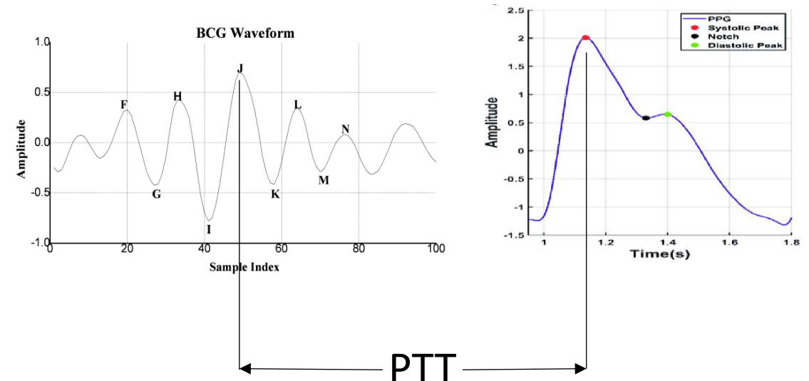
Inbuilt IMU to detect BCG
