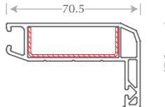
Architrave Profile code: PA-UO-05
