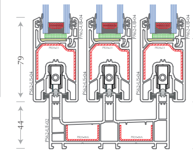
3 Track 3 Panel Sliding Door
