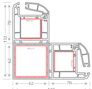
Square Post Assembly
