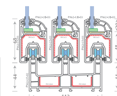
3 Track 3 Panel Sliding Window
