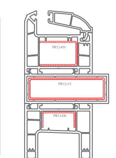
Sliding & Casement Combination Coupler
