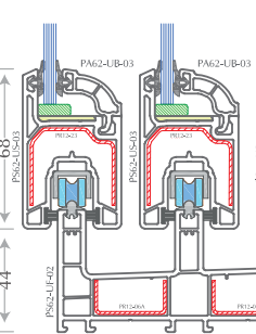
3 Track 2 Panel Sliding Window with Bug Mesh
