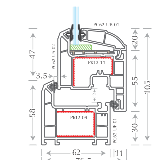
Inward Open and Tilt & Turn Window
