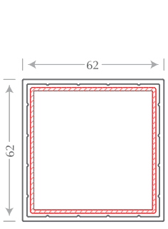
62MM Square POST Profile Code: PA62-UO-01
