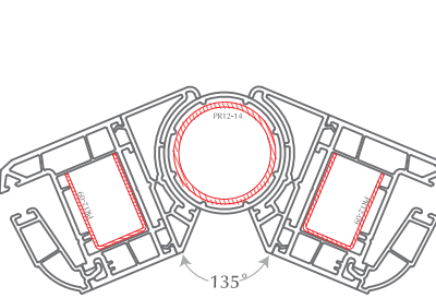
Bay Post Assembly
