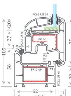
Outward Open Window
