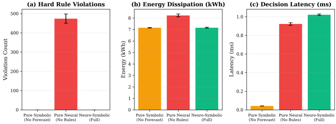
Fig. 6. Experiment C ablation study comparison across safety, energy, and latency.
