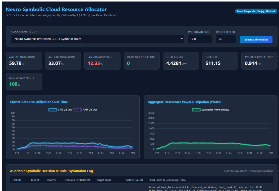
Fig. 7. Demo Dashboard Home Interface, showcasing policy and workload controls.
