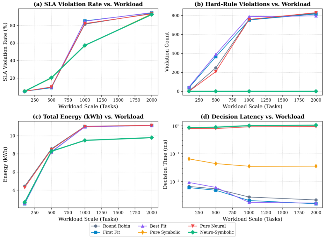
Fig. 5. Experiment B scalability curves across increasing task volumes.
