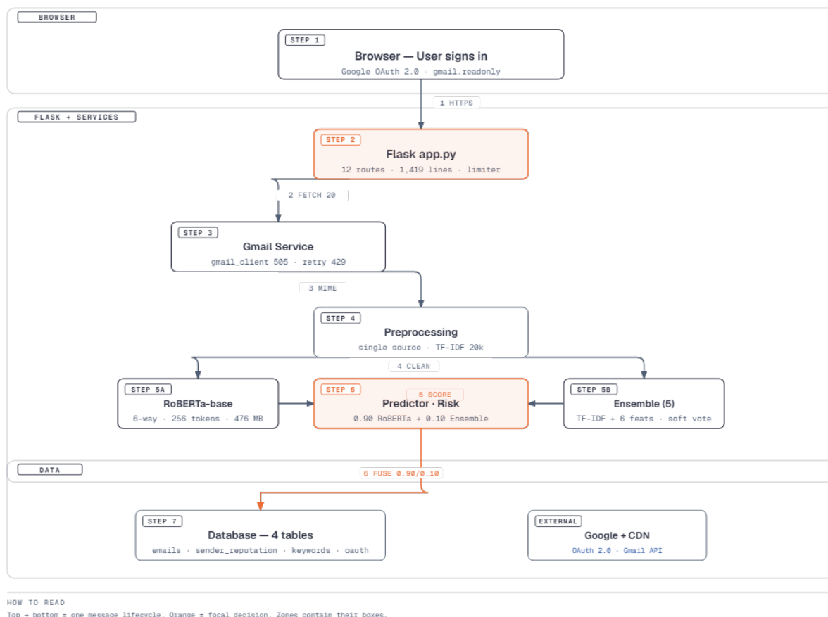
Figure 4.1: System Architecture
