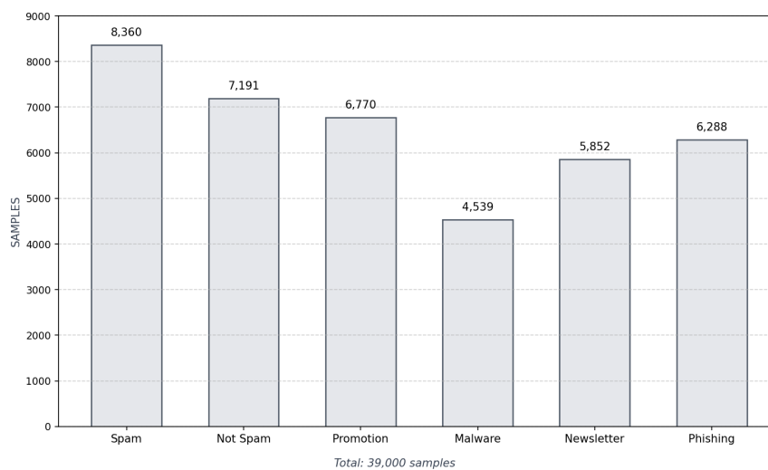
Figure 5.1: Dataset Distribution
