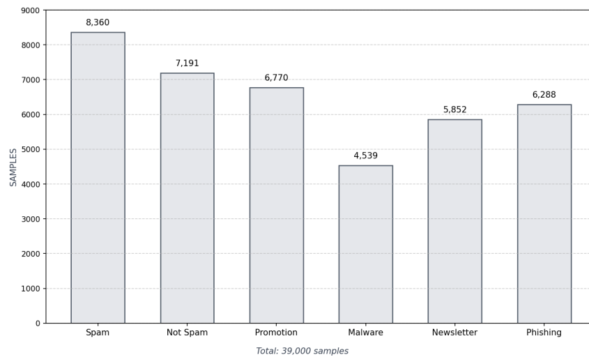
Figure 5.1: Dataset Distribution
