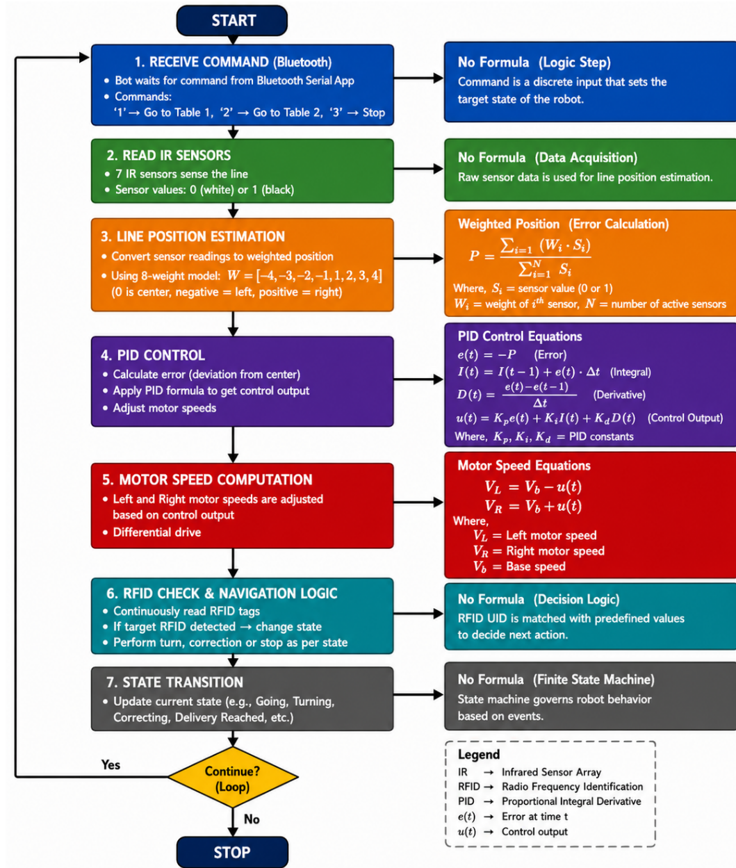
Figure 3. Complete system workflow illustrating Bluetooth command reception, IR-based line sensing, weighted position estimation, PID control, motor actuation, RFID-based decision making, and FSM-based navigation loop.
