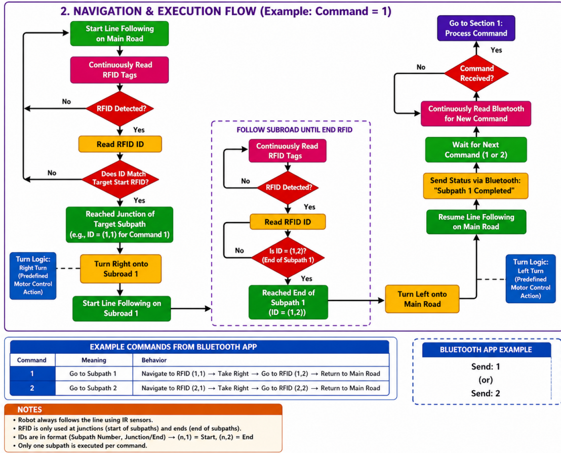
Figure 4. Navigation and execution flowchart for a two-subpath delivery mission (Command = 1 shown). The robot follows the main-road line track until the target-subpath junction RFID tag is detected (ID = (1, 1)), executes a predefined right-turn motor sequence onto the subroad, and continues until the end-of-subpath tag (ID = (1, 2)) triggers a left turn back to the main road. A Bluetooth telemetry message confirms subpath completion; Command = 2 follows an identical structure via RFID pair (2, 1)–(2, 2).
