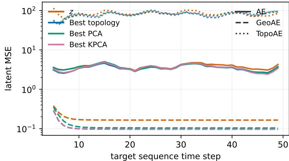
Latent prediction error over time
