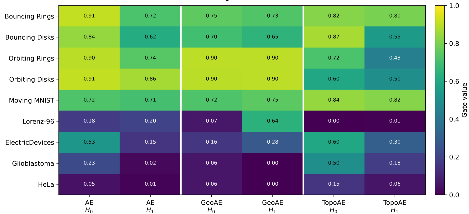
Mean held-out gate values (five seeds)
