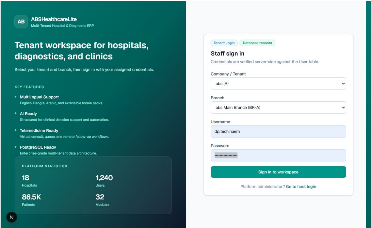
Screen 01 — Staff sign-in surface; any retained password value is masked.
