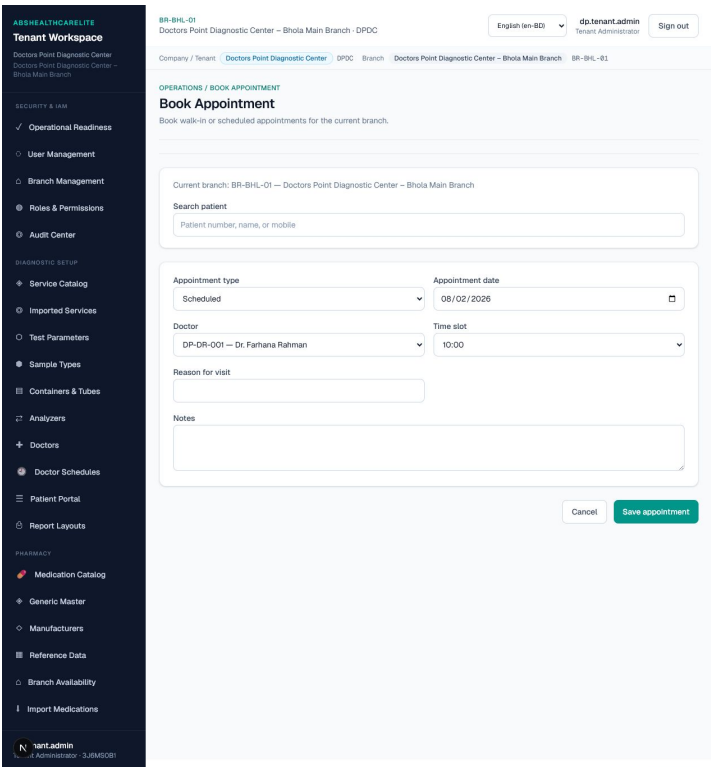
Screen 31 — Published doctor available to appointment booking.
