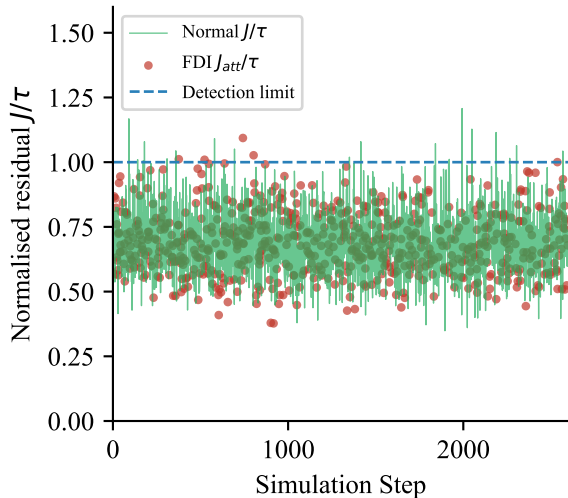
(a) WLS residual: attack evades BDD
