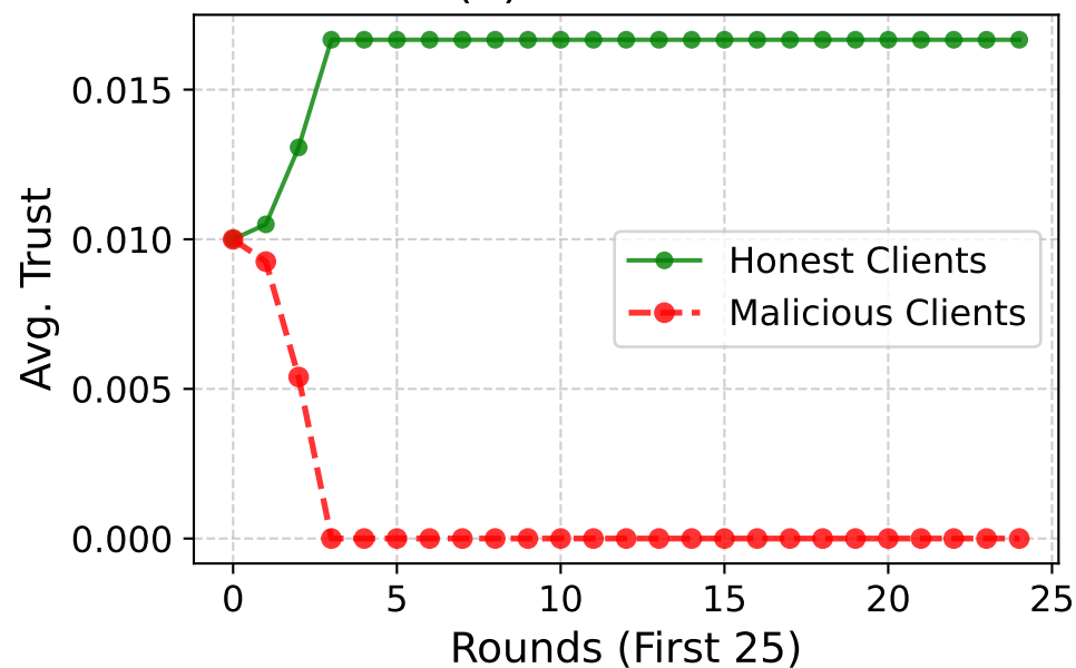
(a) MNIST - IID
