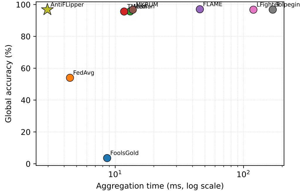
MNIST (Non-IID)
