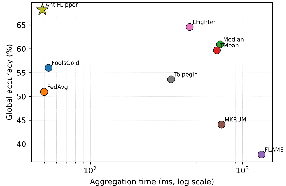
CIFAR-10 (Non-IID)
