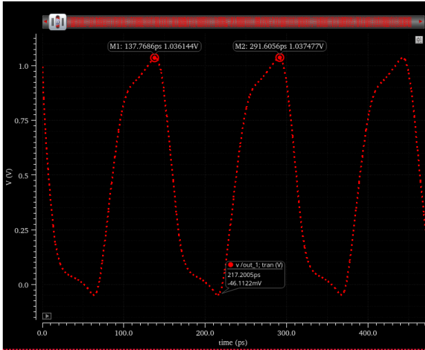
Fig. 4. Post-layout (RC-extracted) transient output waveform showing stable rail-to-rail oscillation at 6.50 GHz with a period of 153.84 ps.
