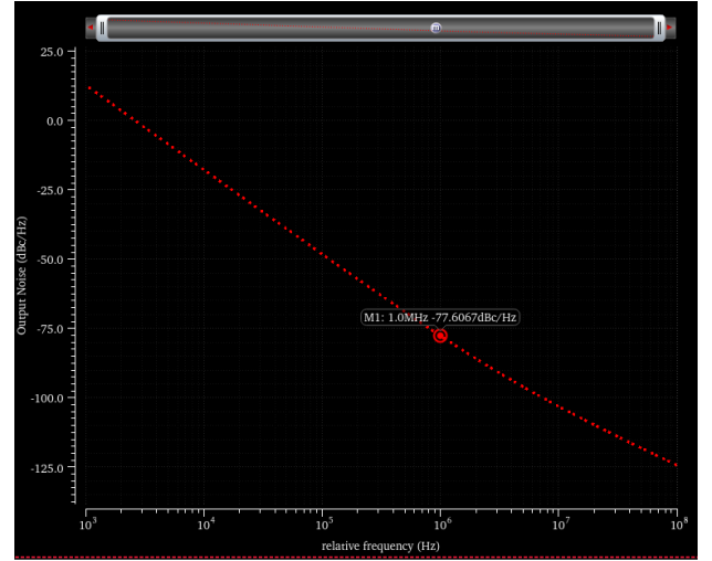
Fig. 5. Post-layout (RC-extracted) single-sideband phase noise versus relative offset frequency, showing -77.6 dBc/Hz at a 1 MHz offset.
