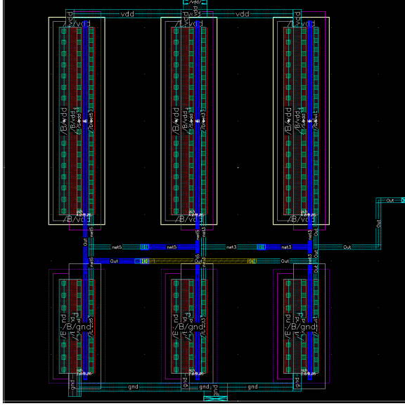
Fig. 3. Manually routed layout core showing row-aligned PMOS and NMOS device matching ( 8.6 \mu\text{m} \times 8.6 \mu\text{m} ).
