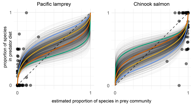
Figure 3: Multi-species functional response, measuring the rate at which California sea lions consume prey as a function of the composition of the prey community. A. Relationship between the proportion of each fish species in the predator diet, measured with gastro-intestinal analysis of euthanized California sea lions, and proportion of each fish species in the prey community, based on the mean posterior estimate of available prey, L_A and S_A for salmon and lamprey, respectively. The credibility intervals for the estimates of available prey, L_A and S_A , are shown in Figure S3. B. Conceptual multi-species functional responses demonstrating how two multi-species functional response curves can have similar local properties in the observed parametric region shown in panel A, yet different global properties due to a large, unobserved parametric region. C. Estimated multi-species functional response, where each black line represents a posterior sample describing the predicted relationship between the expected proportion of each species in the sea lion diet and the proportion of each species in the prey community. Four posterior samples are highlighted in color and are used in Figure 4. The dashed line indicates the 1:1 line, where sea lion consume prey in equal proportion to their abundance in the prey community.
