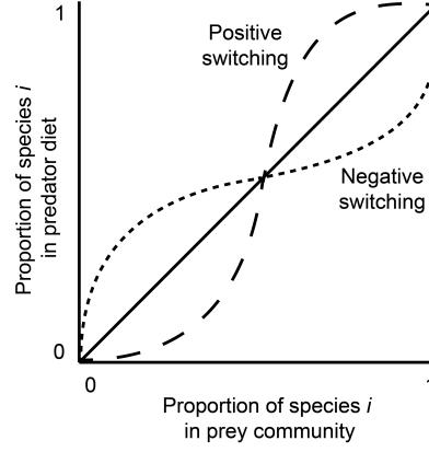
Figure S6. Conceptual diagram of density-dependent multi-species functional response (MSFR), relating the formulation of the density-dependent attack rate (Equations 1-2) to system behavior.
