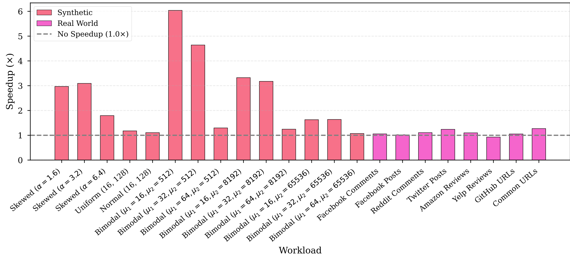
Speedup over libcudf 25.10 (All Workloads)
