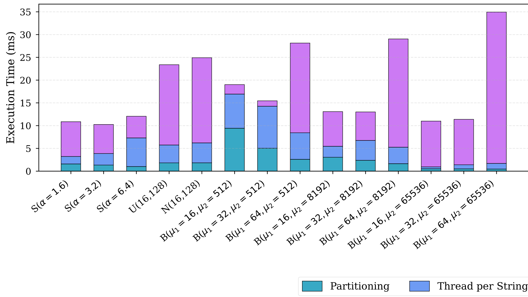
Synthetic Workloads
