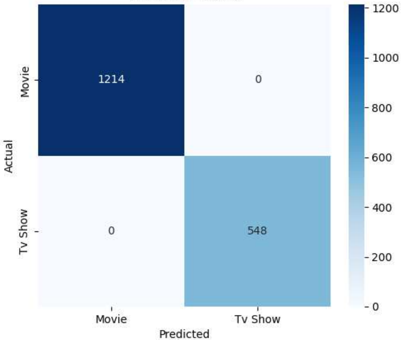
Confusion Matrix
