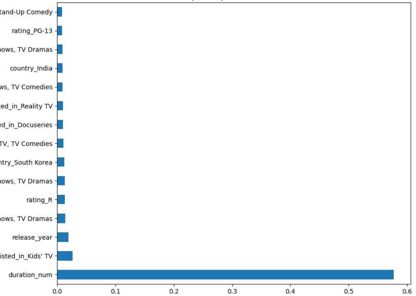
Top 15 Important Features
