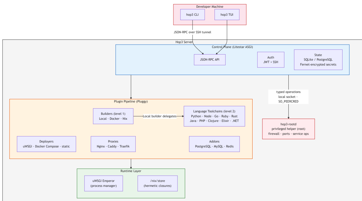
Figure 1: Hop3 system architecture. The CLI and TUI establish SSH tunnels to the server's Litestar ASGI control plane. The plugin pipeline resolves build and deployment strategy dynamically per application, and the runtime layer couples uWSGI process supervision with a Nix store for hermetic closures. The control plane runs unprivileged: host-level operations go through hop3-rootd , a root-owned helper that exposes typed operations over a local socket and authenticates its caller by kernel-supplied credentials (ADR 041, §9.1).
