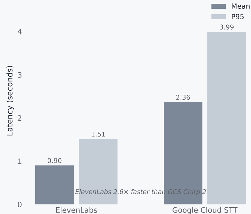
B · Phase 2 provider latency (mean, s)
