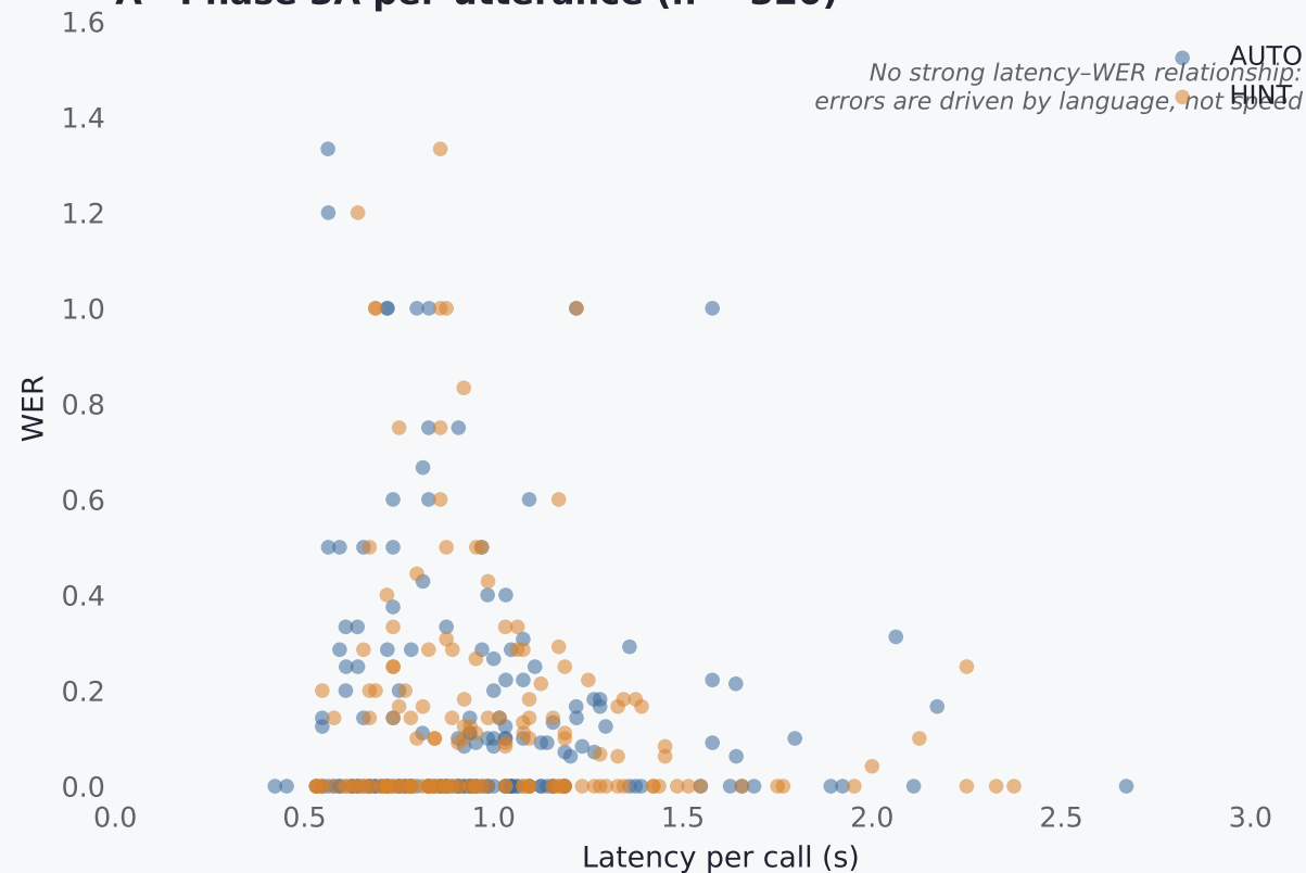
A · Phase 3A per-utterance (n = 320)
