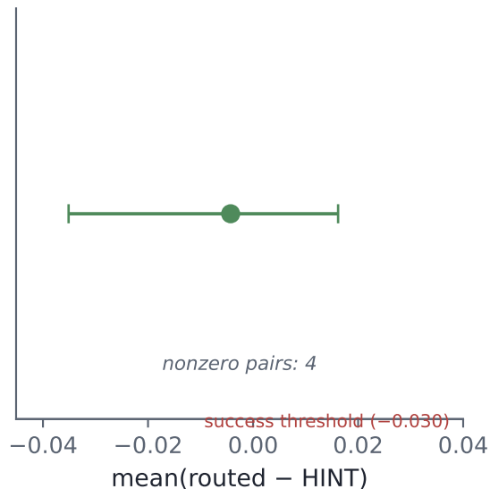
B · Uzbek · \Delta = -0.0043 , p = 0.642
