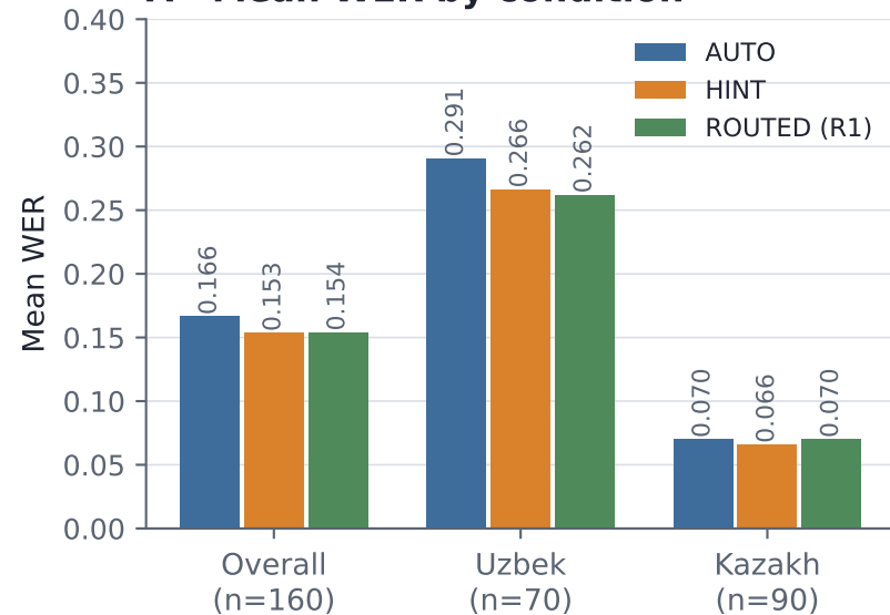
A · Mean WER by condition
