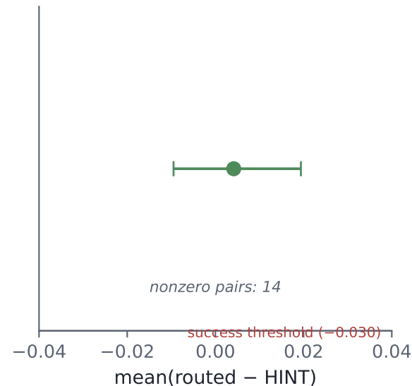
C · Kazakh · \Delta = +0.0042 , p = 0.755
