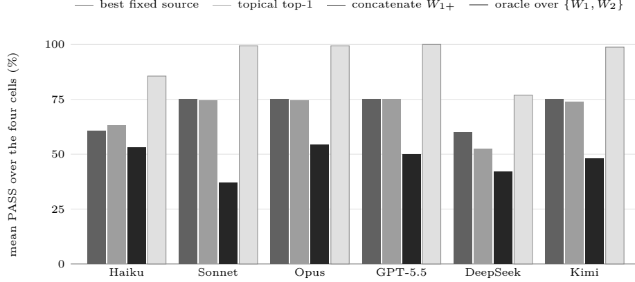
Figure 3: Mean PASS over the four verified cells under the four selection policies of Table 7, per model. Two things are visible that the table states in prose. The two scalar policies land within about a point of each other on most models while failing on different cells, so the ceiling is the policy class rather than the choice of scorer. And concatenating both sources is the worst of the four on every model, below even a fixed single source: refusing to choose costs more than choosing wrongly. The last column reads the per-cell maximum off the test outcomes and is an oracle over the pair, not a router fixed in advance and then evaluated.
