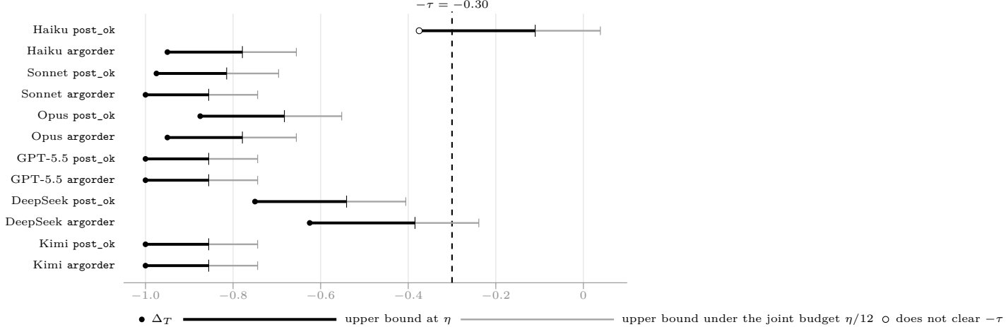
Figure 2: The harm contrast \Delta_T = \text{PASS}_M(W_{1+}, T) - \text{PASS}_M(W_1, T) on both API cells of every model, with the bound that carries the verification. A cell is verified harmful when the upper bound clears -\tau = -0.30 , so a bar ending left of the dashed line is a verified collapse. Thick bars are the marginal bounds at \eta = 0.10 , one family per cell: eleven of twelve clear. Thin grey bars are the same contrasts under a single \eta spread across all twelve, at per-interval level \eta/12 : ten clear, and every model keeps at least one. The one cell that never clears is Haiku’s api_post_ok , whose W_1 arm is depressed by an omitted import rather than by the contract (§7.5.1). Values are those of Table 5, recomputed from the released per-cell counts.
