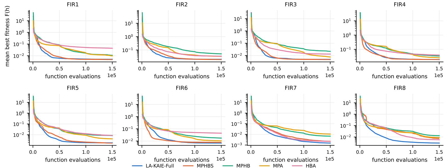
FIR: mean convergence over paired runs
