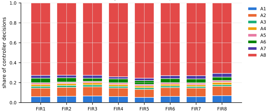
LA-KAIE-Full: exchange-action distribution per instance
