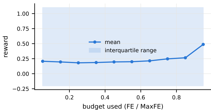
reward evolution
