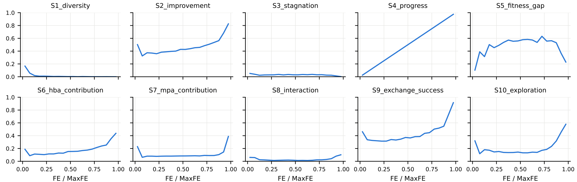
LA-KAIE-Full: mean landscape-state trajectories (all instances)
