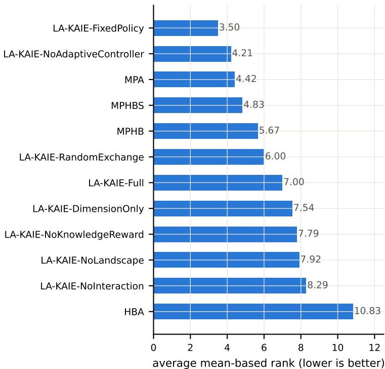
CEC2022: average ranks (all methods)
