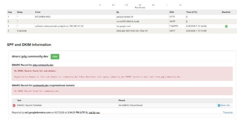
Figure 4: Verification of SPF, DKIM, and DMARC cryptographic records
