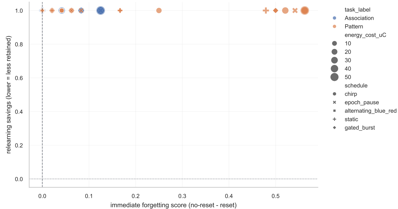
Forgetting versus savings
