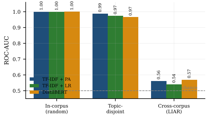
Fig. 10. ROC-AUC of each model across three evaluation regimes: in-corpus random split, in-corpus topic-disjoint split, and cross-corpus transfer to LIAR. Ranking quality survives topic shift within ISOT but collapses to near-chance on an independently constructed corpus. The dashed line marks chance (0.5).
