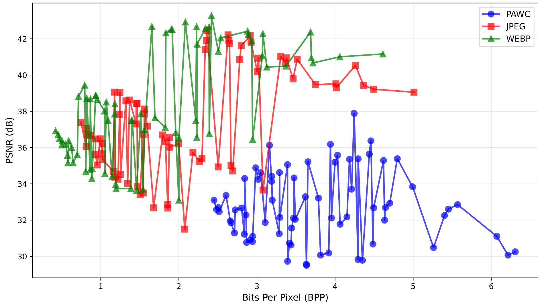
Rate-Distortion Performance (Kodak Dataset)
