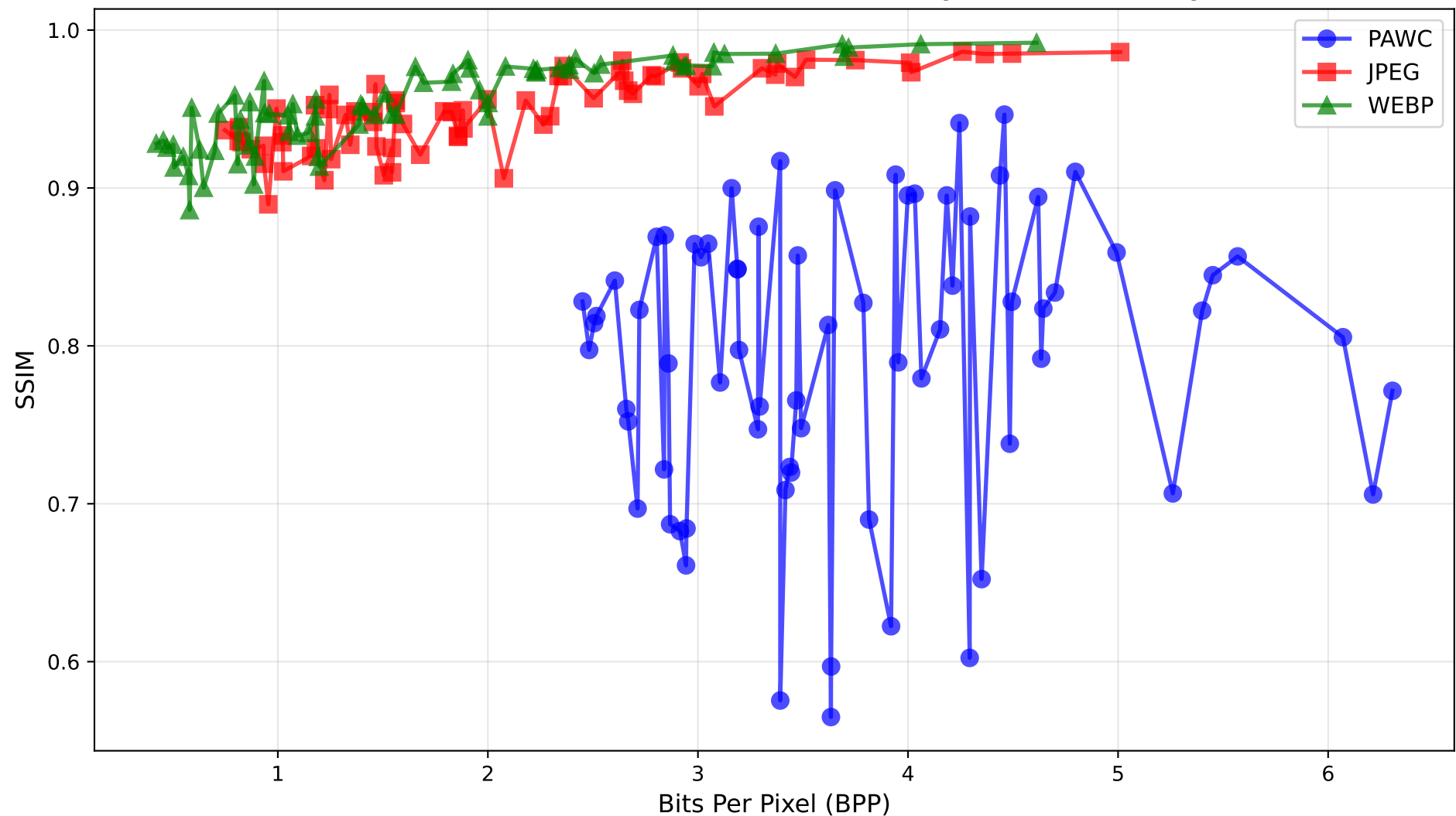
Rate-Distortion Performance - SSIM (Kodak Dataset)
