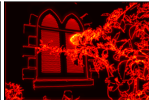
Fused ( \mathcal{I} )
