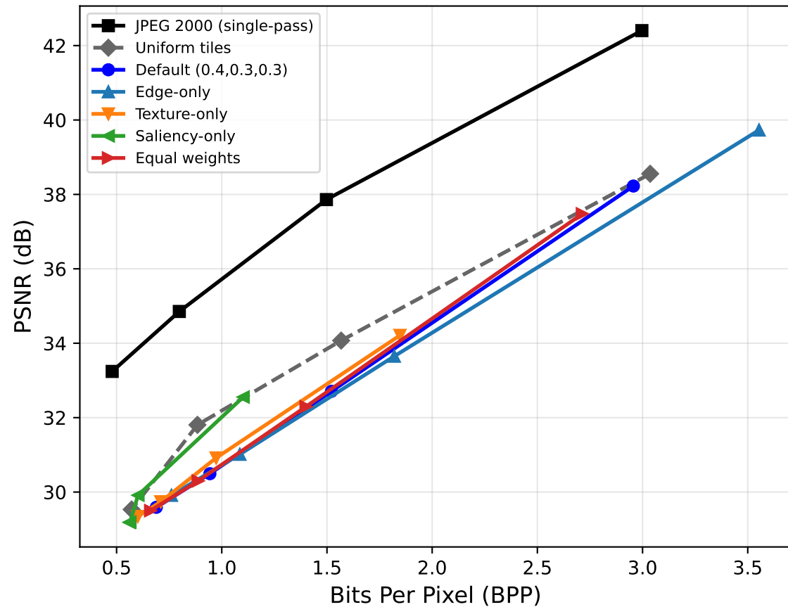
Global fidelity
