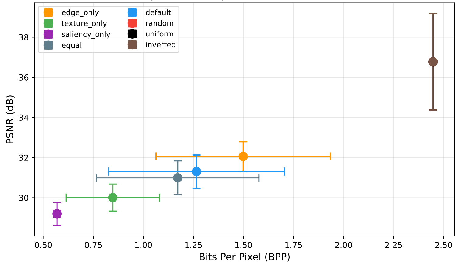
Ablation: Importance Map Variants on Kodak (Q70, n=24)
