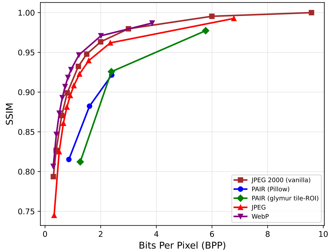
Rate-Distortion (SSIM)
