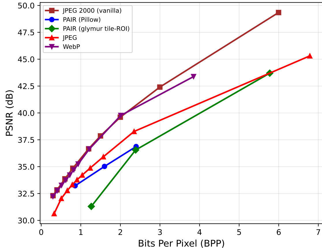
Rate-Distortion (PSNR)
