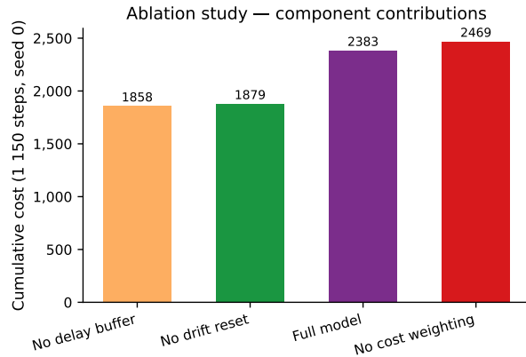
Fig. 3. Bar chart comparing cumulative cost across the four ablation variants. no_cost and full are dramatically more expensive than no_drift and no_delay , isolating cost weighting as the dominant factor.
