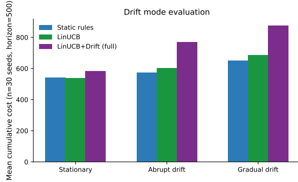
Fig. 7. Grouped bar chart of mean cumulative cost by drift mode \times policy. linucb_with_drift_full is uniformly worst; linucb_with_drift_no_reset is visually indistinguishable from linucb .
