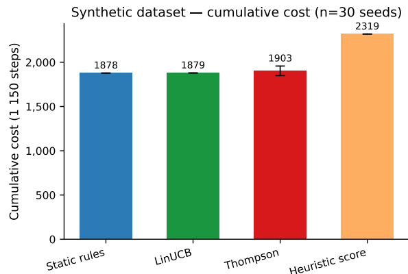
Fig. 1. Cumulative cost per policy on the synthetic dataset (n=30 seeds, error bars = \pm 1 std).
