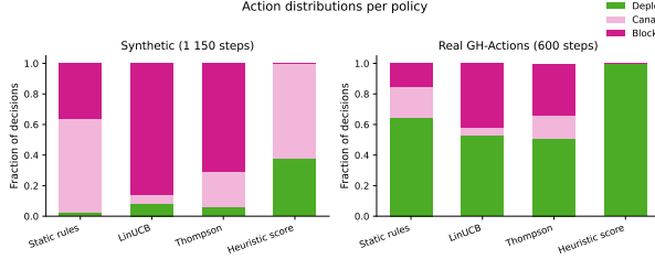
Fig. 5. Stacked-bar action distribution (deploy/canary/block) for all policies on synthetic (left) and real (right) datasets.
