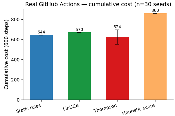
Fig. 4. Cumulative cost per policy on real GitHub Actions data (n=30 seeds, error bars = \pm 1 std).
