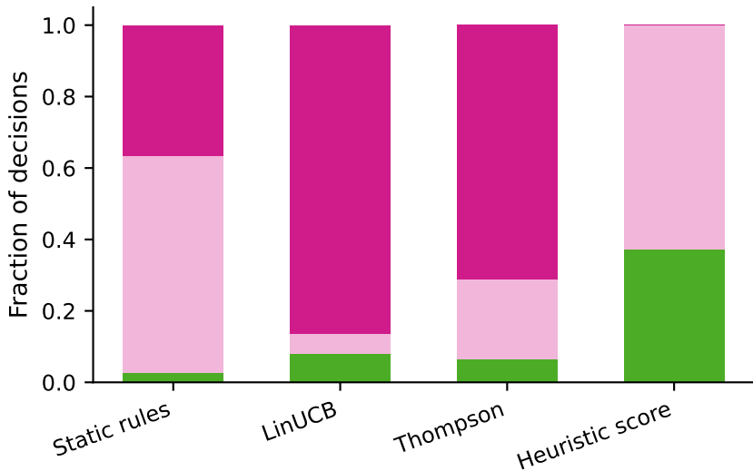
Synthetic (1 150 steps)
