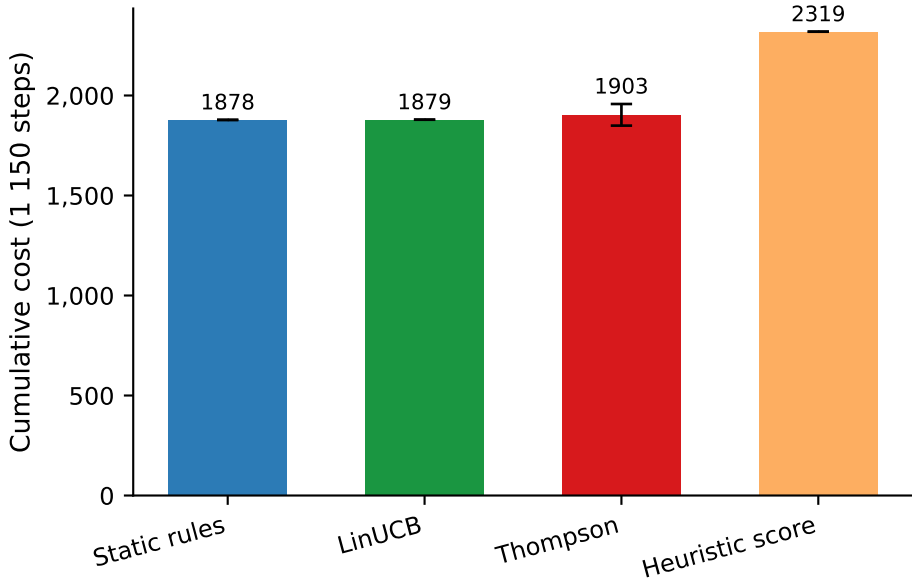
Synthetic dataset — cumulative cost (n=30 seeds)
