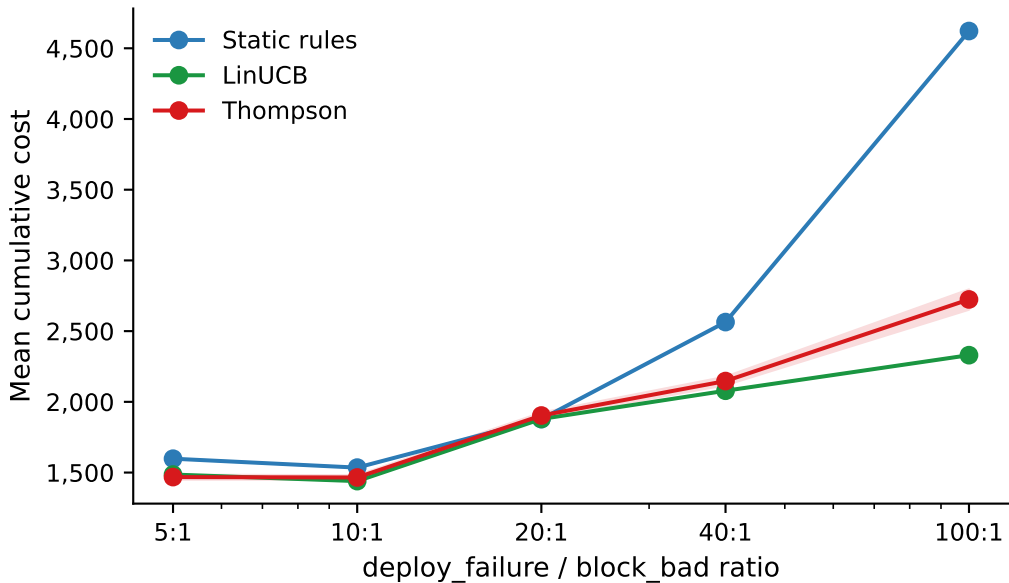
Cost-ratio sensitivity sweep (n=30 seeds)
