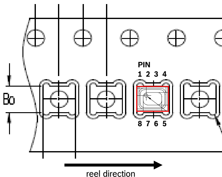
Figure 22: Orientation within tape
