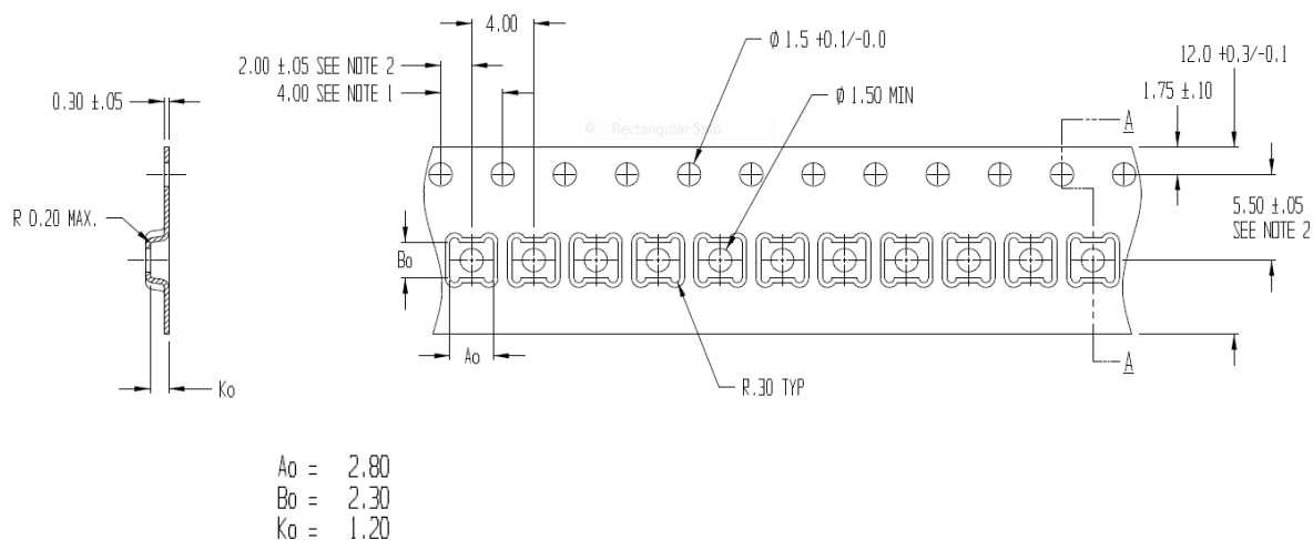
Figure 21: Tape and Reel dimensions
