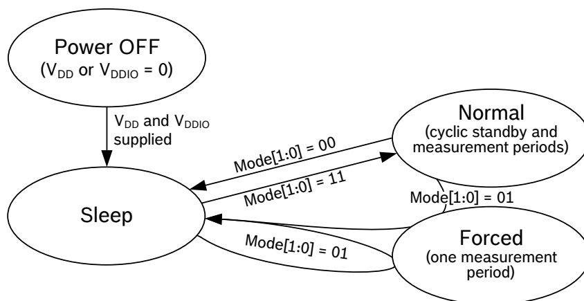
Figure 5: Mode transition diagram
