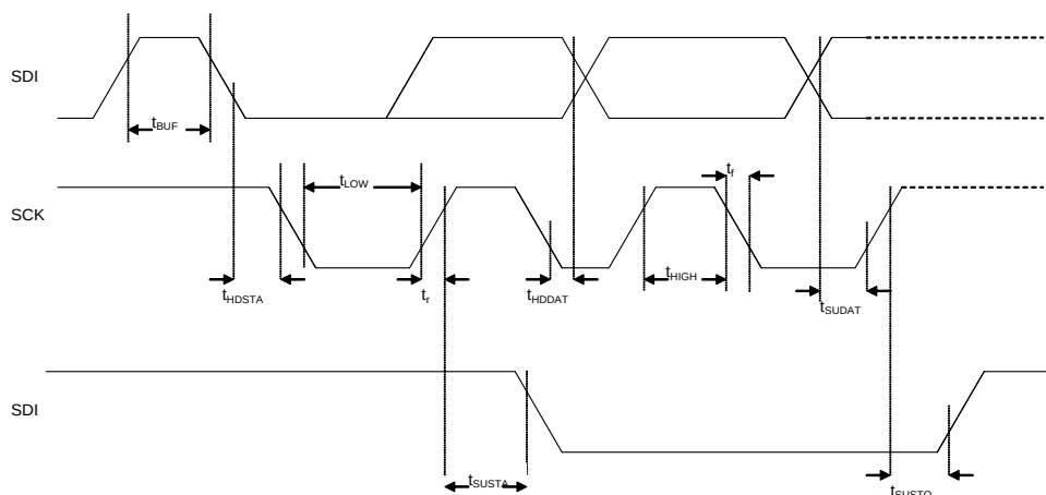
Figure 12: I²C timing diagram
