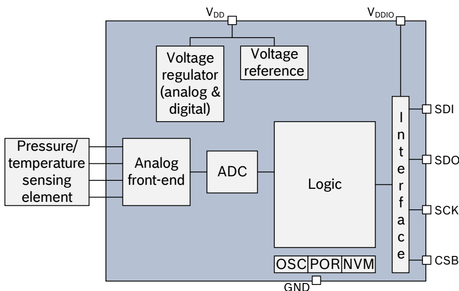
Figure 1: Block diagram of BMP280
