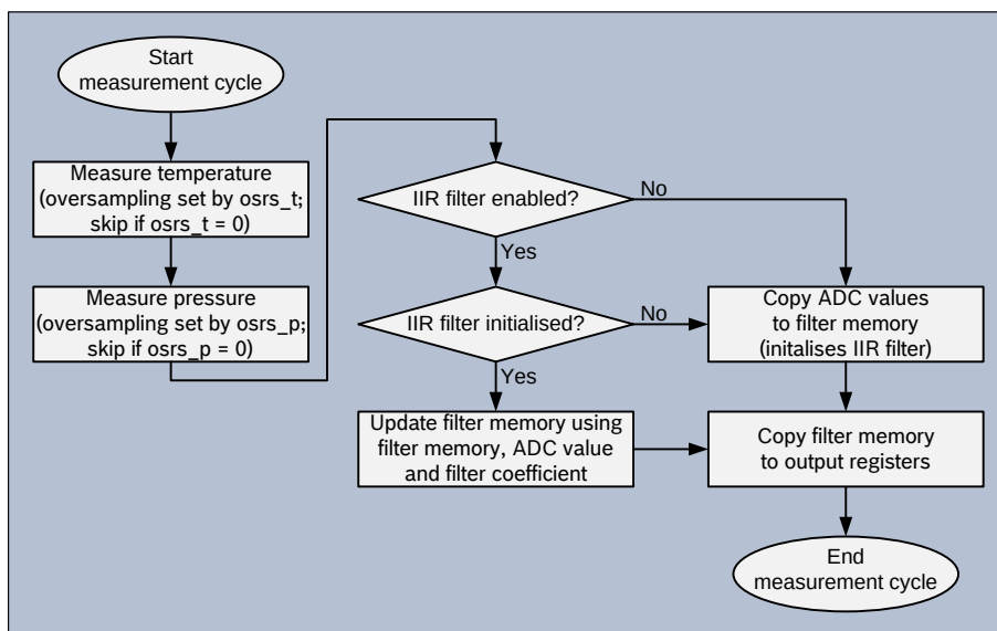
Figure 2: BMP280 measurement cycle
