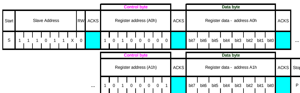
Figure 7: I 2 C multiple byte write (not auto-incremented)
