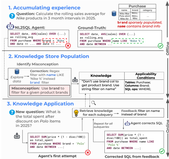
Figure 1: Example workflow of Tk-Boost.
