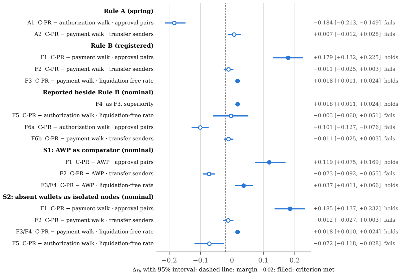
FIGURE 2. Contrasts fixed by Rules A and B and by the registered sensitivity analyses, with 95% paired-bootstrap intervals (400 resamples, seed 42). Filled markers: criterion met; open markers: not met. The dashed line is the non-inferiority margin of -0.02 . Only A1–A2 and F1–F3 decide a rule; the other verdicts are nominal and unadjusted.
