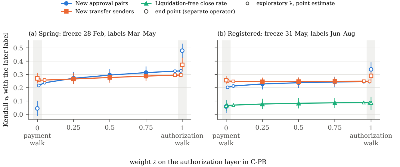
FIGURE 3. Kendall \tau_b of C-PR with each later label against the authorization weight \lambda . Filled markers with 95% paired-bootstrap intervals are the registered grid \lambda \in \{0.25, 0.5, 0.75\} ; open markers with intervals at \lambda = 0 and \lambda = 1 are the payment and authorization walks, separate operators that the line does not join; small open markers at \lambda \in \{0.01, 0.05, 0.95, 0.99\} are exploratory point estimates. (a) Spring holdout; the trader label was defined only for the registered window, so this panel has no trader curve. (b) Registered window. Values are in Table 3 and Appendix A.
