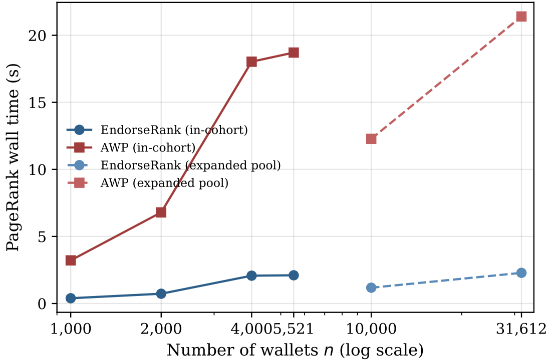
Figure 4.4: PageRank wall-clock runtime versus cohort size (log x -axis). Solid lines: in-cohort scaling on the matched GMX sample ( n \leq 5,521 ). Dashed lines: expanded wallet pool ( N = 31,612 ). EndorseRank remains approximately 9–10 \times faster than AWP at n = 10,000 ( \approx 10.4\times ) and at full pool size ( \approx 9.4\times ).
