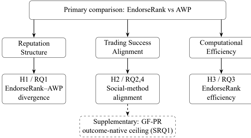
Figure 2.3: Conceptual model: primary EndorseRank vs. AWP comparison mapped to reputation structure (H1/RQ1), social-method alignment (H2/RQ2–4), and computational efficiency (H3/RQ3). GF-PR (dashed) is a supplementary outcome-native ceiling reference (SRQ1), not a third peer social method.
