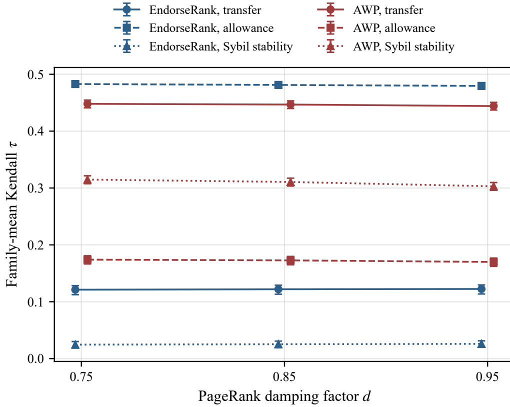
Figure 4.4: Damping sensitivity of the family-mean Kendall \tau of EndorseRank and AWP on the transfer, allowance and Sybil-stability families across d \in \{0.75, 0.85, 0.95\} , with 95% bootstrap intervals (values from Table 4.6; matched cohort, n = 27,844 contracts).
