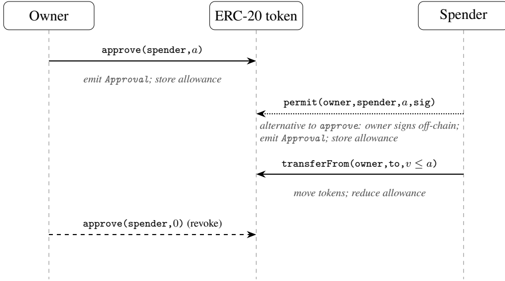
Figure 2.1: ERC-20 allowance lifecycle: approve , or its signature-based alternative permit (dotted), an optional transferFrom , and revoke . An EndorseRank edge sums, over tokens, one term for the most recent Approval event of its owner–spender pair in the observation window, and the term weights that approval by its age and amount as AWP weights a transfer. A later approval replaces an earlier one.
