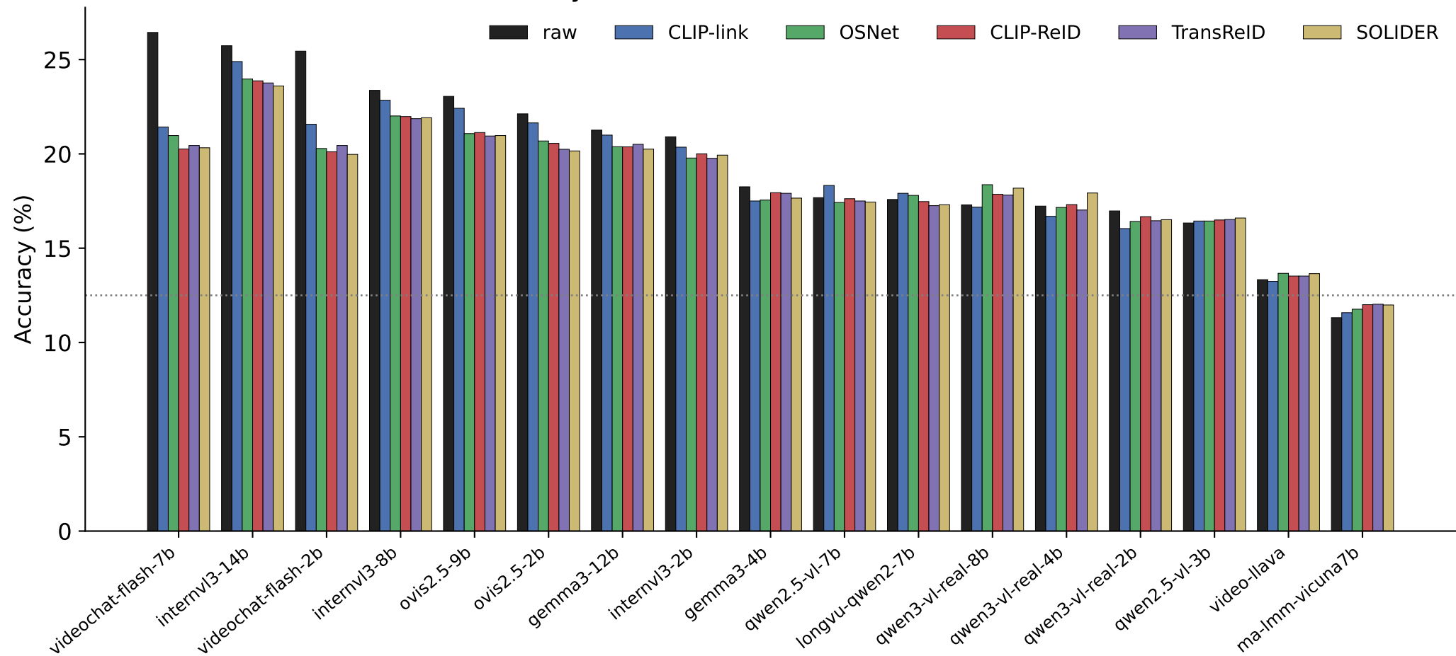
Per-VLM accuracy: raw vs. tracker+ID-method (chance 12.5%)
