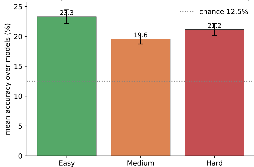
Difficulty calibration: labels track real model accuracy
